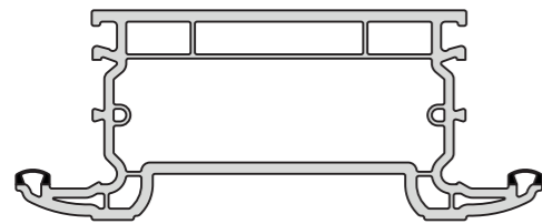
LPD084 Midrail
