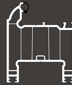
MBF092 Sash
