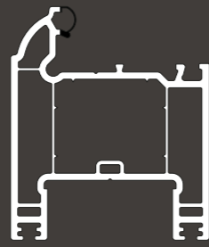
LBF092 Sash
