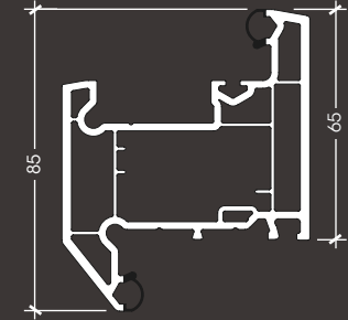
LRW022 Transom Z
