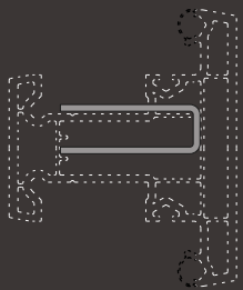
LRW122 Transom Steel Reinforcement
