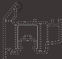
LRW133 Sash Reinforcement
