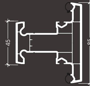
LRW021 Transom T
