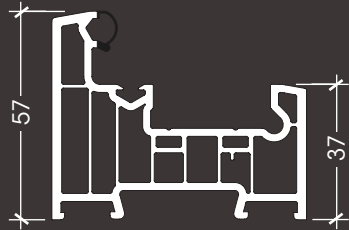
LRW012 Outer Frame
